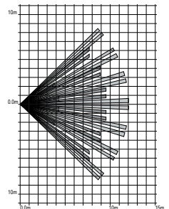
XCELRPT coverage
