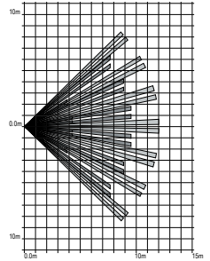
XCELWPT coverage
