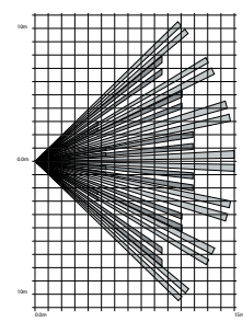
XCELR coverage
