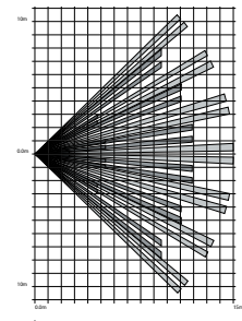
XCELW coverage
