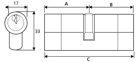
Fortress 3 Star BS Double Euro Profile Cylinder
