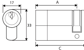
Fortress 3 Star BS Single Euro Profile Cylinder
