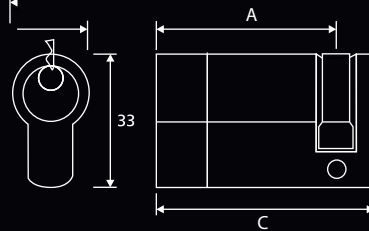
Fortress 3 Star BS Double Euro Profile Cylinder
