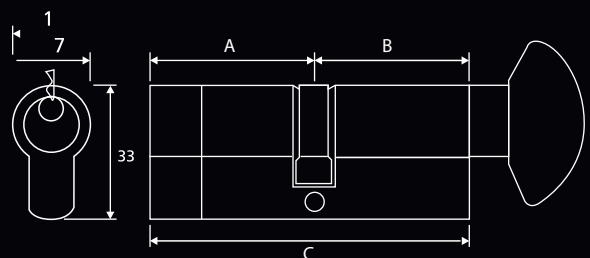
Fortress 3 Star BS Double Euro Profile Thumbturn Cylinder
