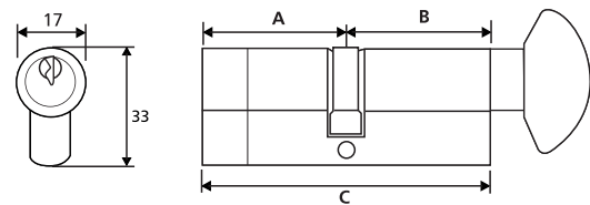
Fortress 3 Star BS Double Euro Profile Thumbturn Cylinder
