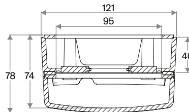
Top View (40 mm Spacer)
