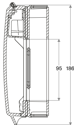
Surface Mount Side View (40 mm Spacer)
