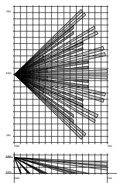
XCELW coverage
