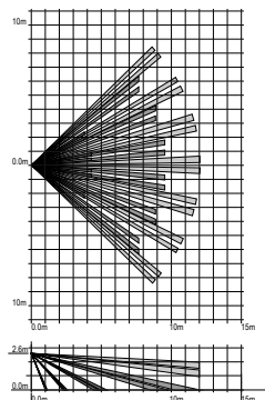
XCELRPT coverage
