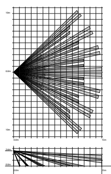
XCELR coverage
