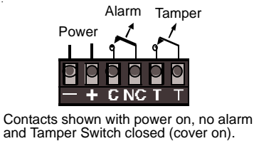
Board Layout
