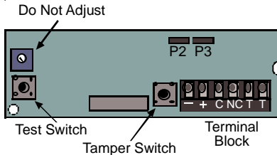
Board Layout
