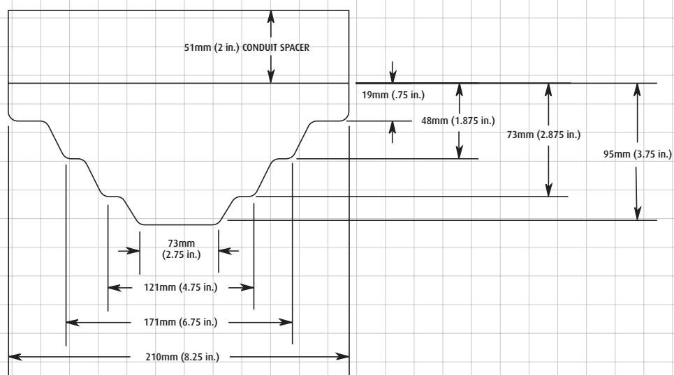
DEPTH CHART OF THE POLYCARBONATE DETECTOR STOPPER
