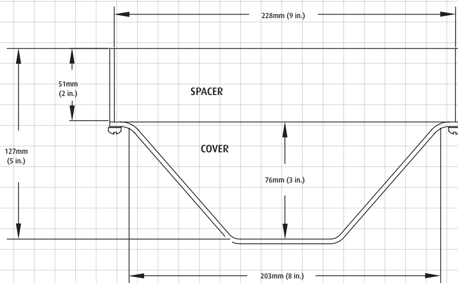
DEPTH CHART OF THE STEEL SMOKE DETECTOR STOPPER
