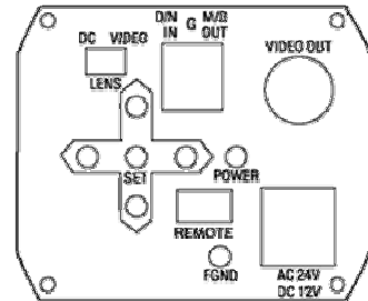
rear panel
